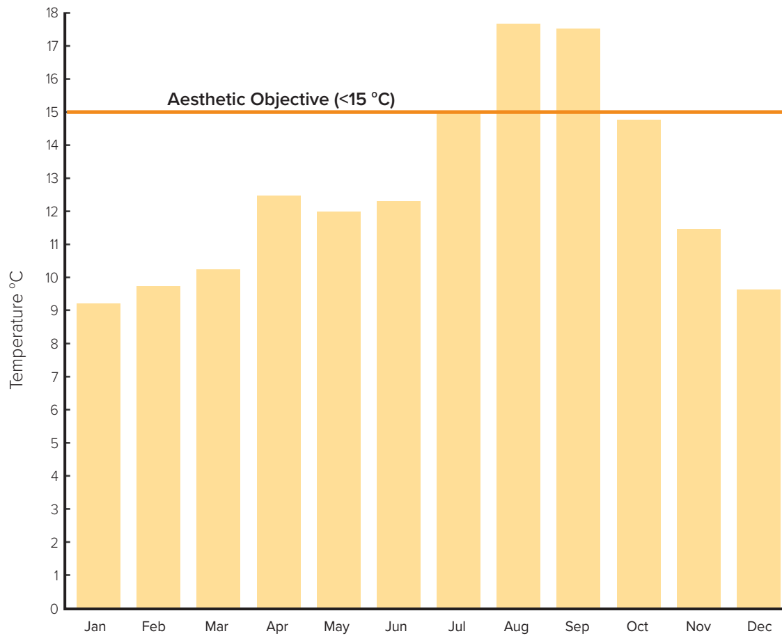
Figure 4 – 2023 Average Monthly Water Temperatures in the Distribution System
