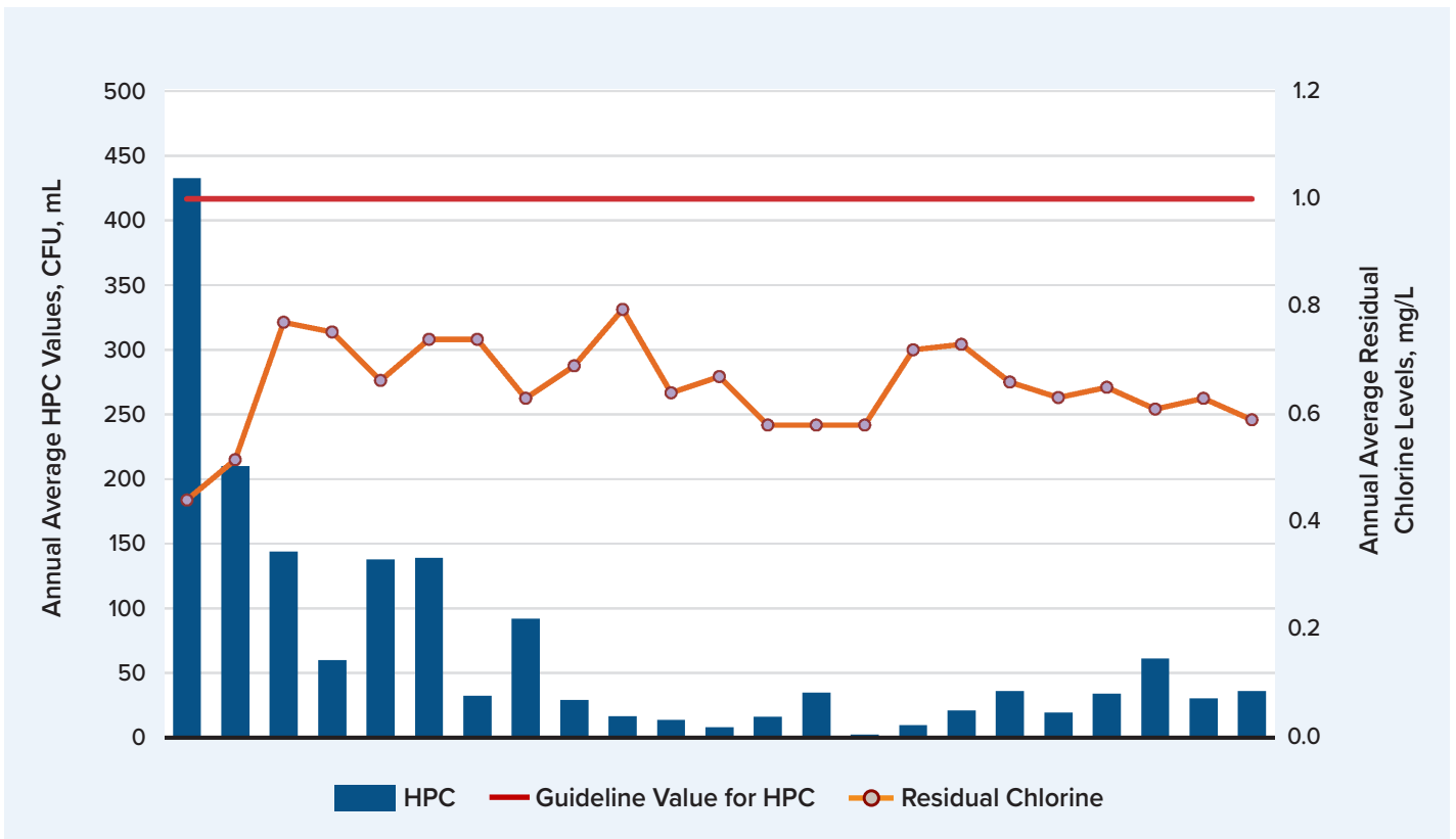
Figure 6 – Improvements in Drinking Water Distribution System (1998-2023)
